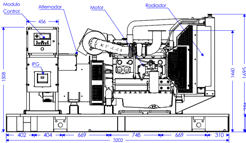
VISTA FRONTAL
